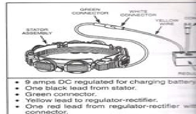
Fig. 3 - 9 Amp DC Regulated Stator
