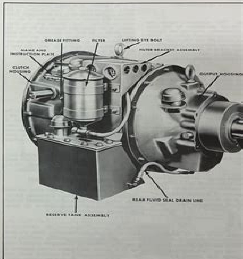
Figure 2. Model CO-10,000 & 11,500 Series Three-Stage Torque Converter (3/4 Rear View).
