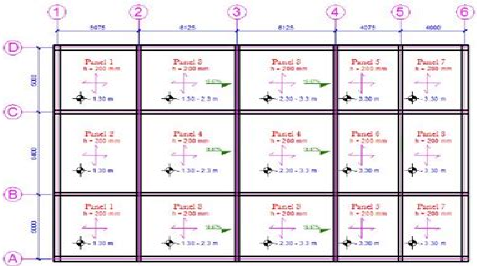
Figure 8.6: Preliminary General Arrangement of the Pool Hall
