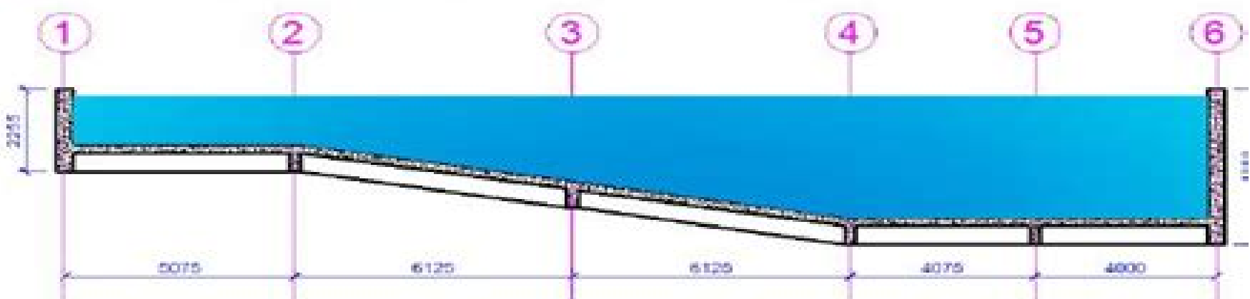
Figure 8.7: Proposed Longitudinal Section through the Pool Hall
