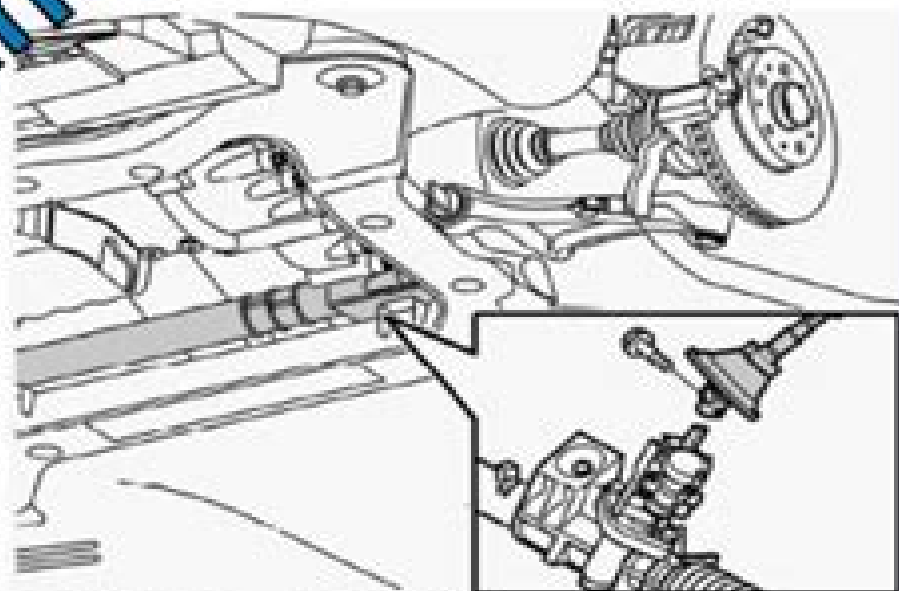
Fig. 106: Identifying Steering Wheel Shaft Joint Courtesy of VOLVO CARS OF NORTH AMERICA.
