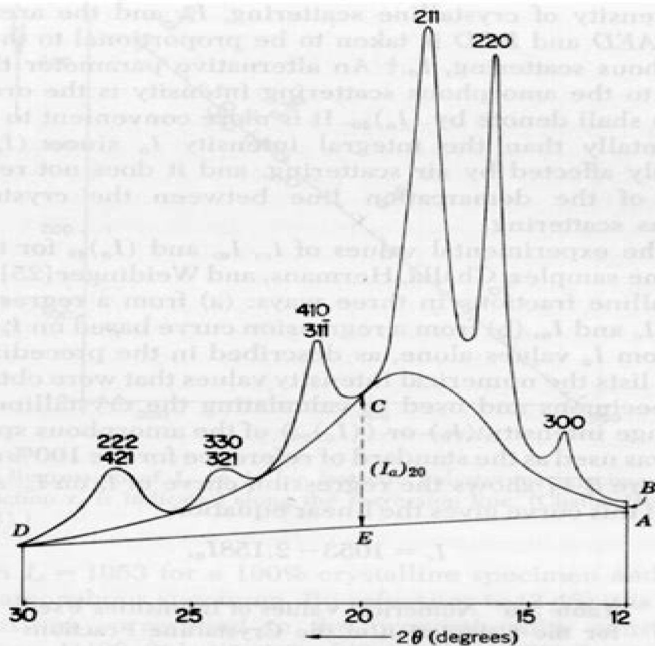
Figure 3-15 X-Ray scattering curve of a partially crystalline isotactic polystyrene specimen. (Challa, Hermans, and Weidinger [25].)
