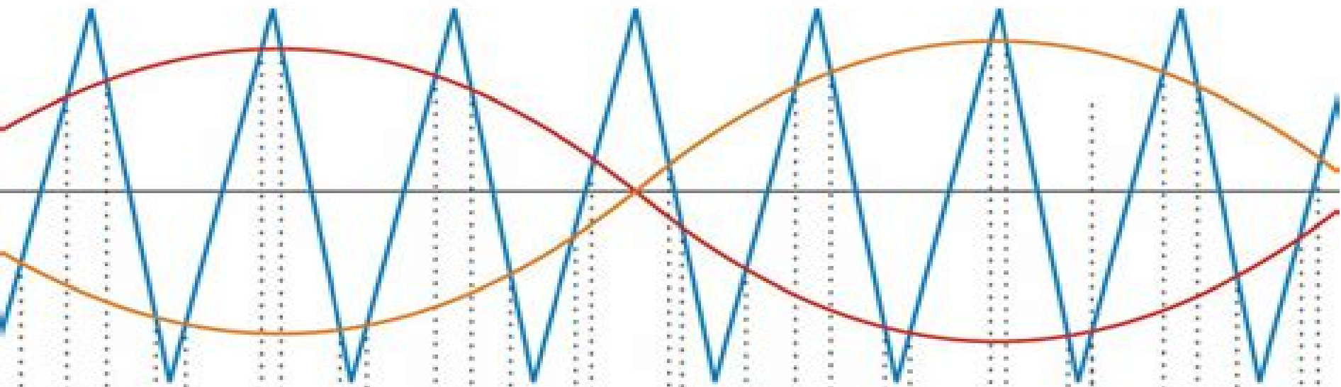
(b) S1/S4 PWM pulses
