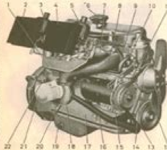
Fig. 16. The engine (right side)
