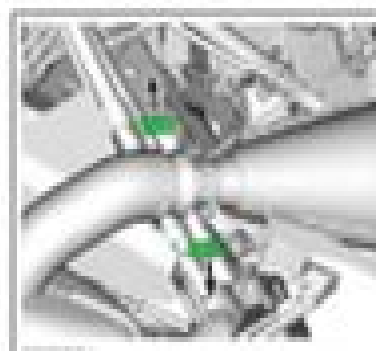
4. Disconnect the press fasteners from the muffler GTS.
