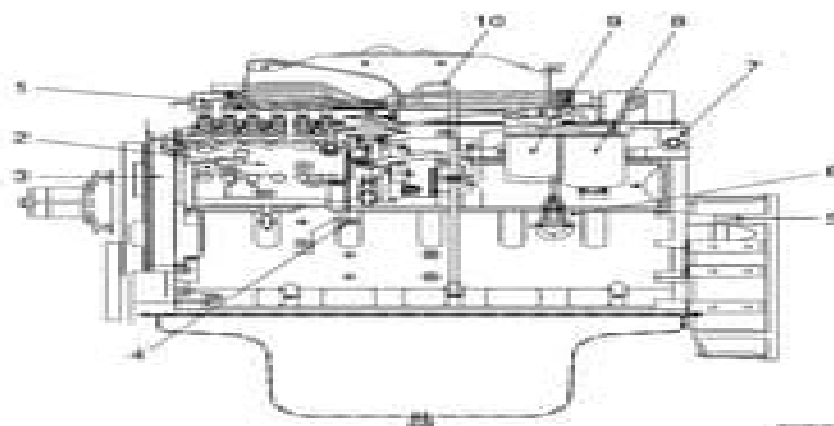
Figure 1 Engine, structure(EC210)
