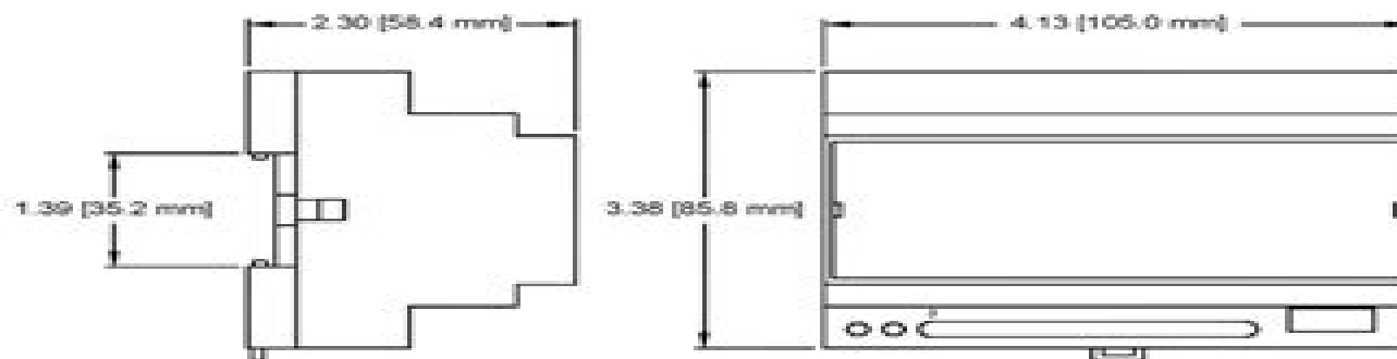
Figure 1 Enclosure Dimensions
