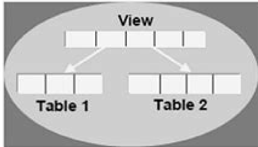
ABAP Dictionary
