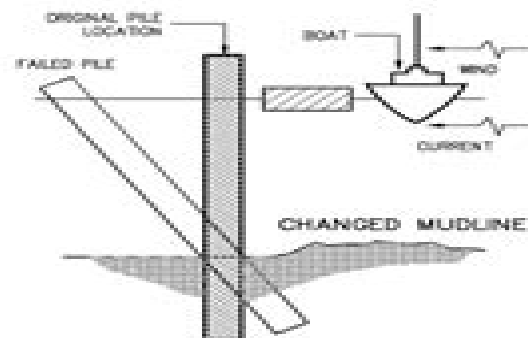
PILE FAILS WITH SOIL (not enough penetration)
