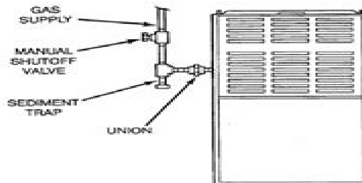
Fig. 7—Typical Gas Pipe Arrangement
