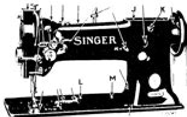
Fig. 2 Front View of Machine Showing Oiling Points and Adjustments
