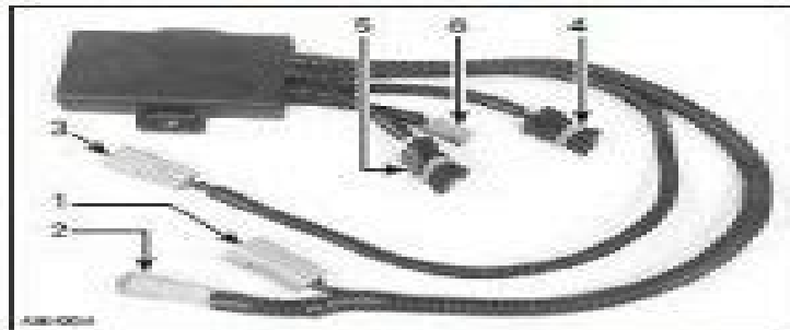
TYPICAL — BOMBARDIER 290 W MPEM — NON-REV MODELS 1. High tension coils, 4-00 housing 2. Generating coils (low and high speed), 4-00 housing 3. Trigger coil, 4-00 housing 4. DESS switch, 4-00 housing 5. DESS pre-amp and ignition coil, 4-00 housing 6. Atmospheric pressure sensor, 4-00 housing
