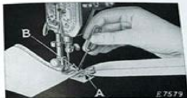
Fig. 64. Adjusting the Binder.
