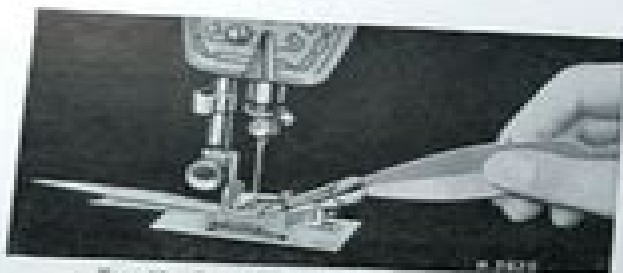
Fig. 62. Inserting Binding in Binder.
