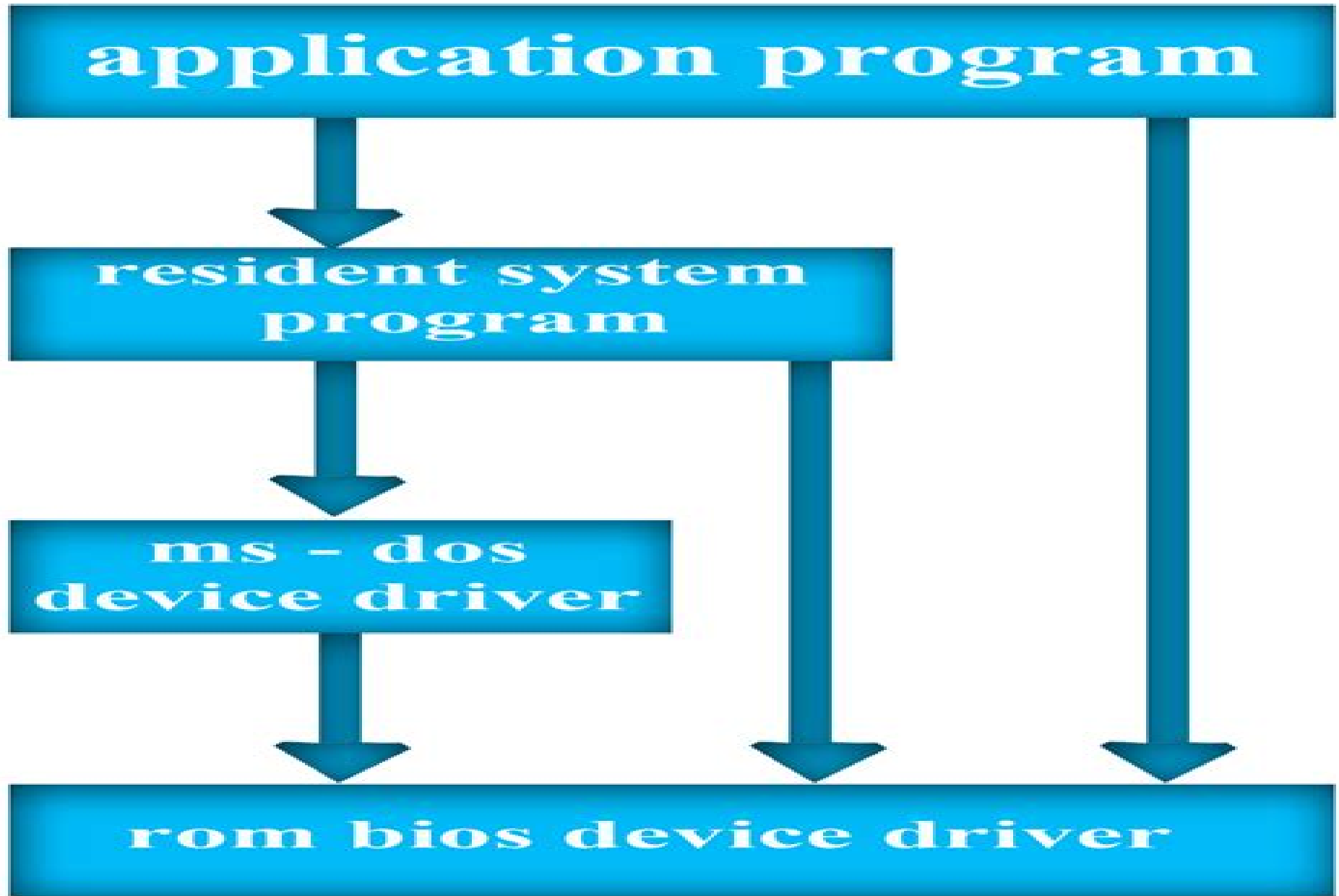
ms dos system structure
