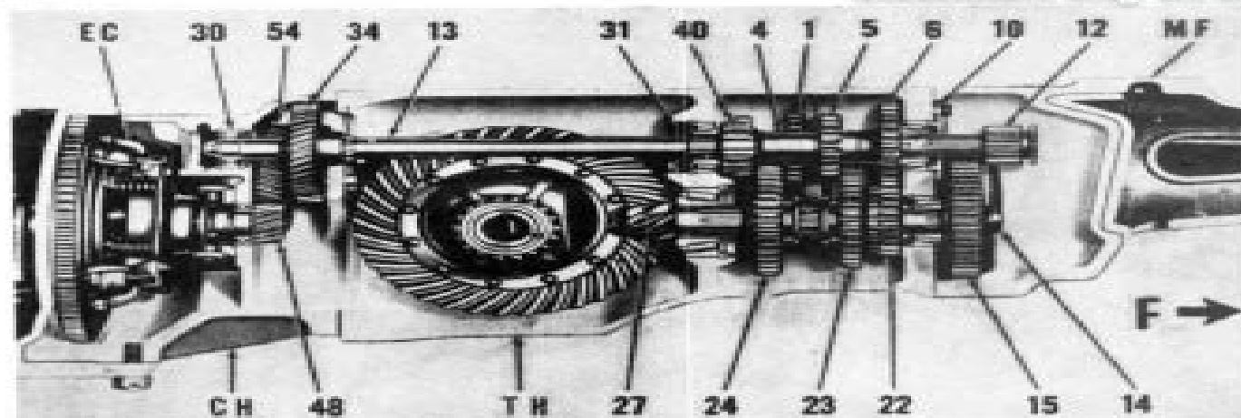
Fig. AC96—Model G transmission shafts, bevel pinion, ring gear, and differential unit are contained in the transmission housing.
