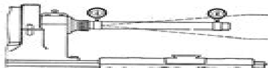
Spindle Alignment—Vertical Plane
