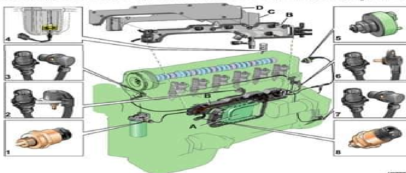
Figure 1 DOWNLOAD SERVICE MANUAL D12C. Engine sensors (some have dual functions)
