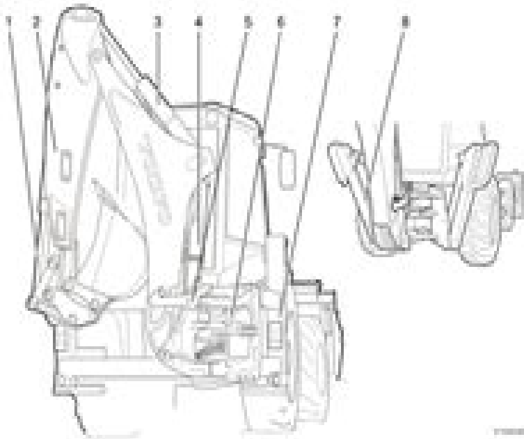
Figure 1 Location of cylinders on the backhoe unit
