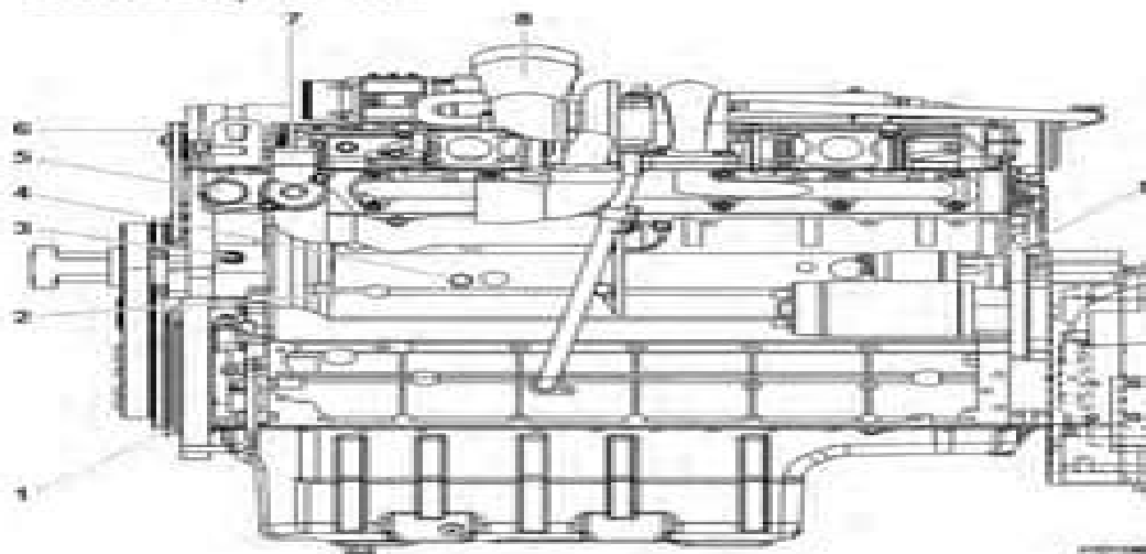
Figure 1 Engine, start motor side view
