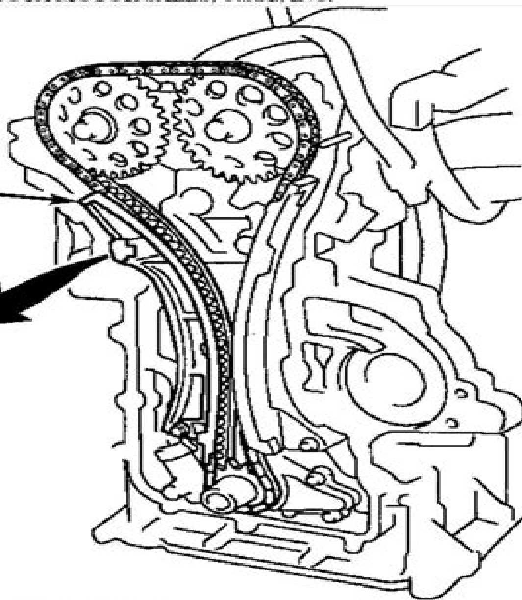
Fig. 29: Installing Timing Chain, Timing Chain Tensioner Slipper & Crank Angle Sensor Plate Courtesy of TOYOTA MOTOR SALES, U.S.A., INC.
