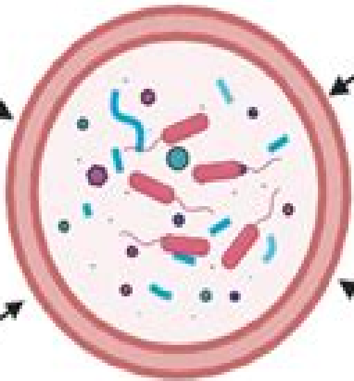
Membrane fouling
