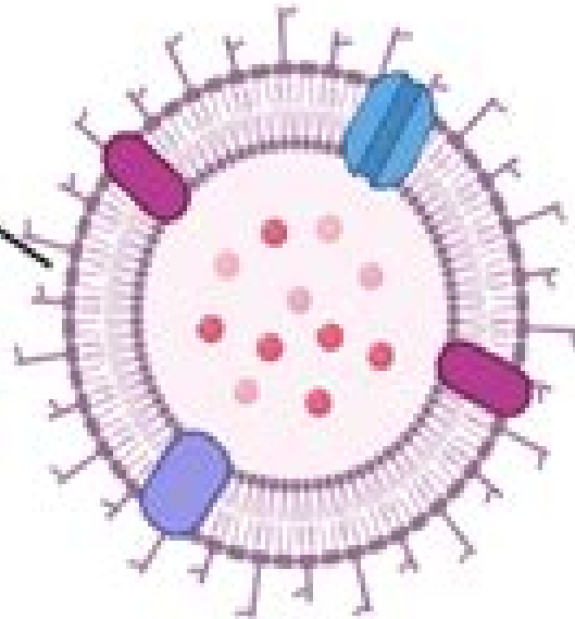
Organic fouling
