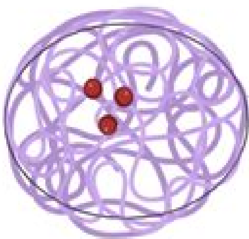
Inorganic fouling
