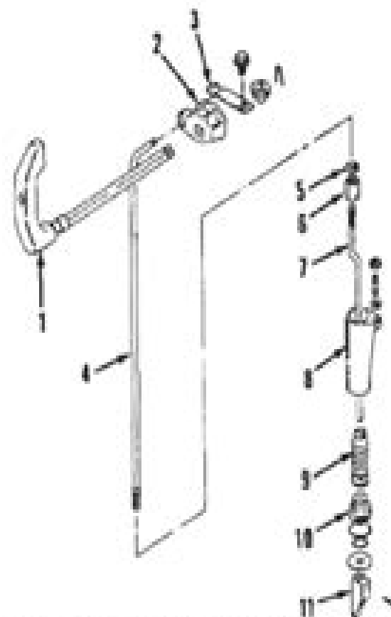
Fig. S26-35—Exploded view of shift control linkage components.
