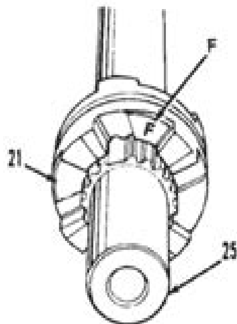
Fig. S26-34—Install clutch (21) on propeller shaft (25) with mark (F) facing forward gear.
