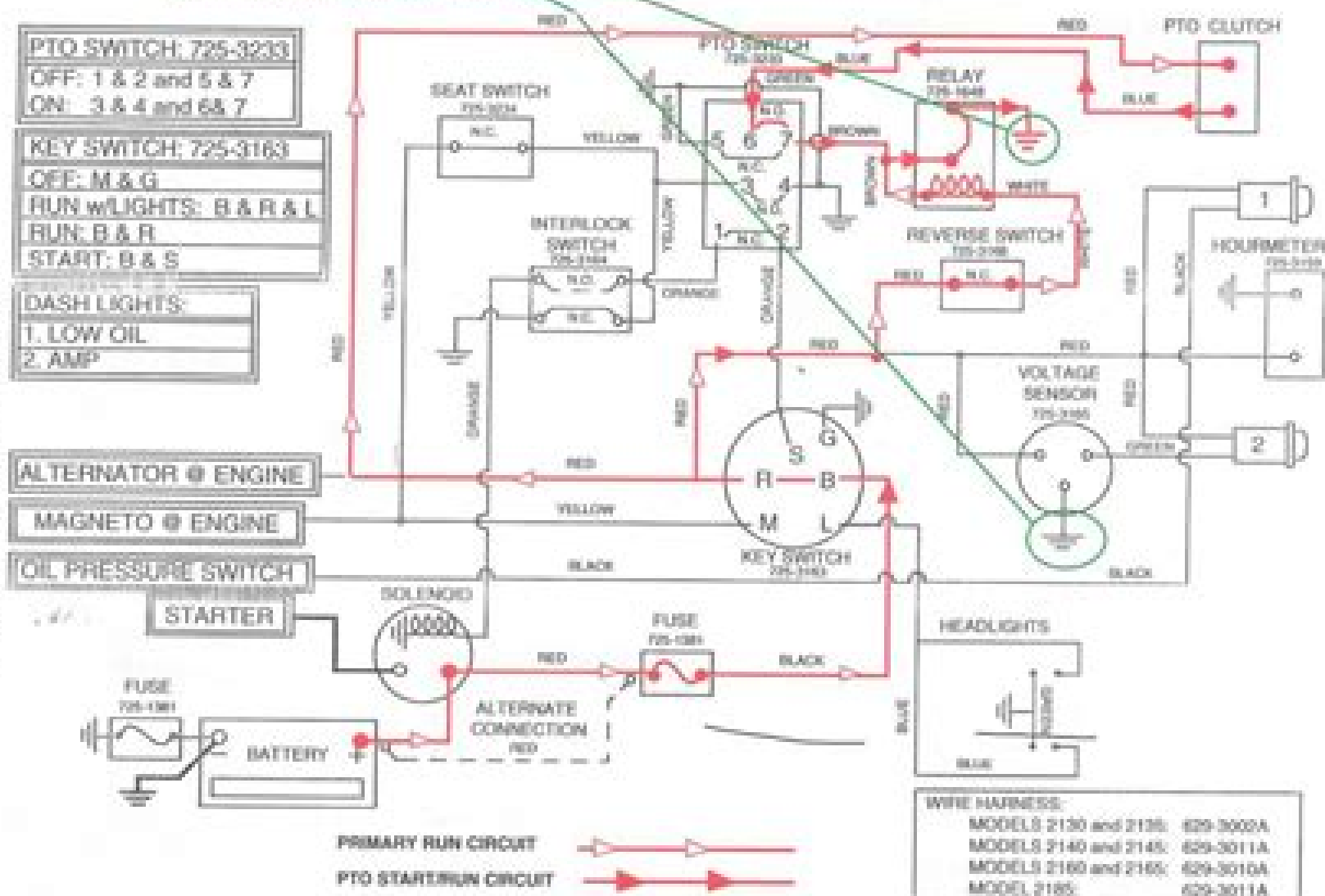
Figure D-6. PTO Start/Run, All Models. D-12
