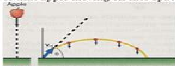
Figure 10.1 Motion of an apple or a projectile.
