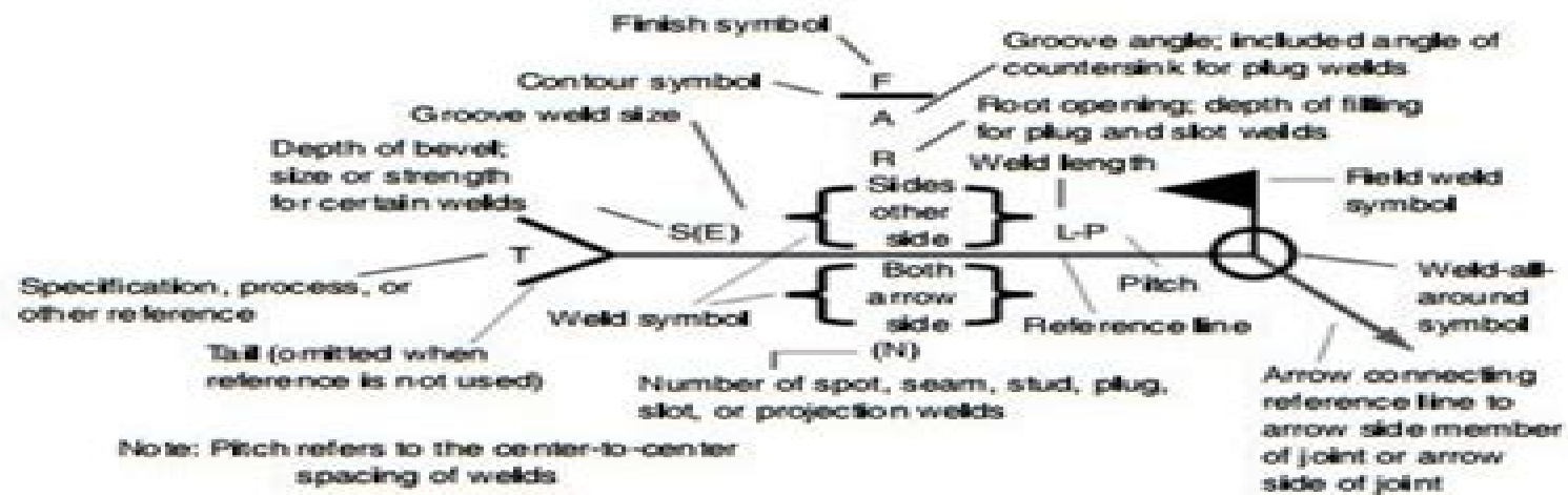
Figure 7.17 Welding symbols can include a wide variety of information
