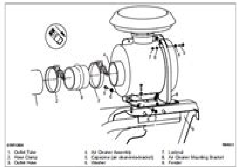
Fig. 1. Air Cleaner Assembly (Front view)
