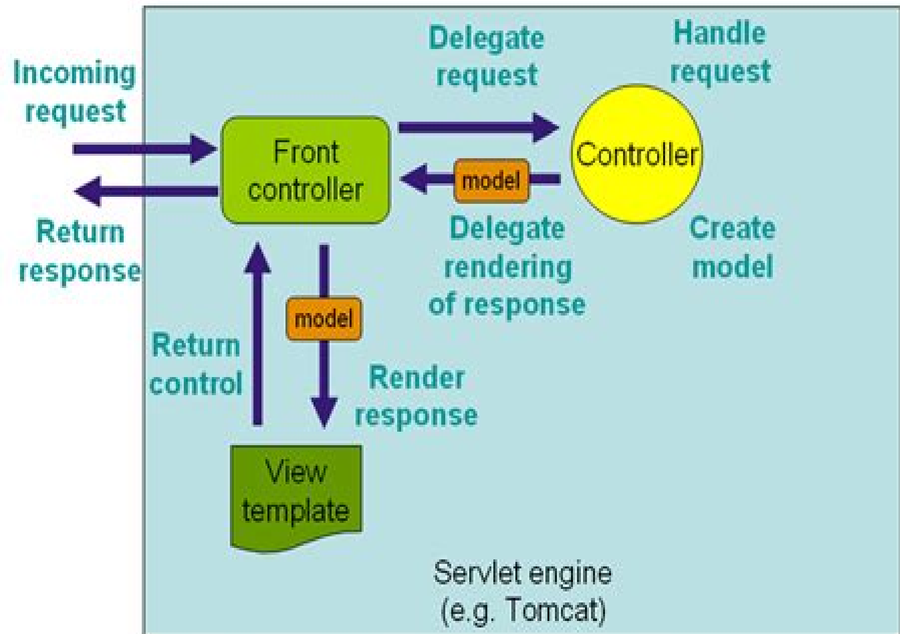
The requesting processing workflow in Spring Web MVC (high level)
