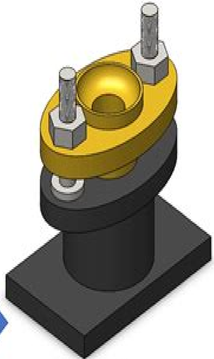
Stuffing Box
