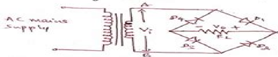
Fig.2. Circuit diagram of a FWBR
