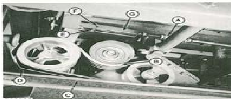
A—Turnbuckle B—Drive Belt C—Mounting Bolt D—Belt Guide E—End Plate F—Gauge Hole G—Spring Guide
