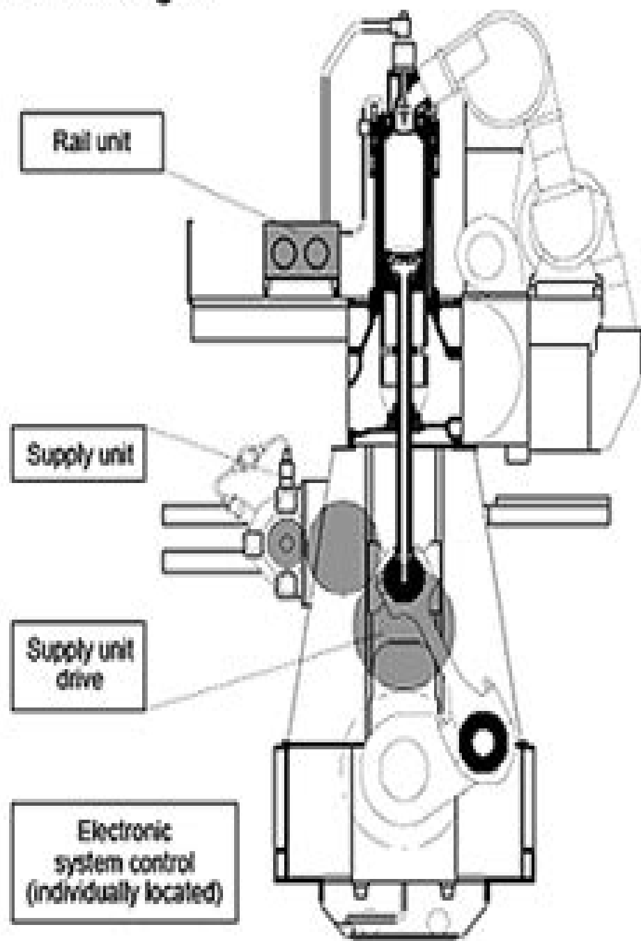
RT-flex engine
