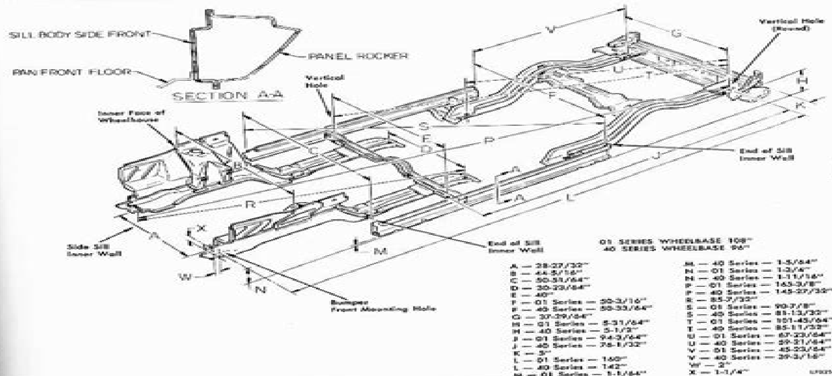
FIGURE 1 — 01 and 40 Series Frame Dimensions
