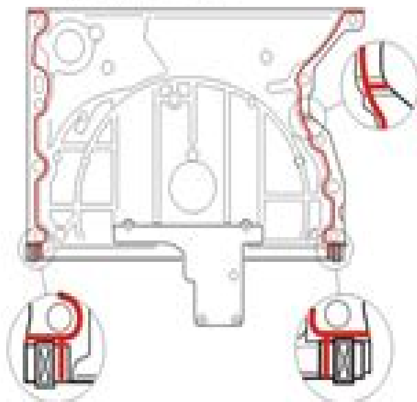
Base of silicone PPS 1161231
