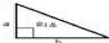
Heron's Formula
