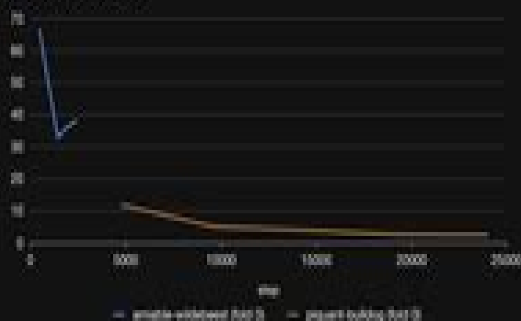
VALIDATION MAE
