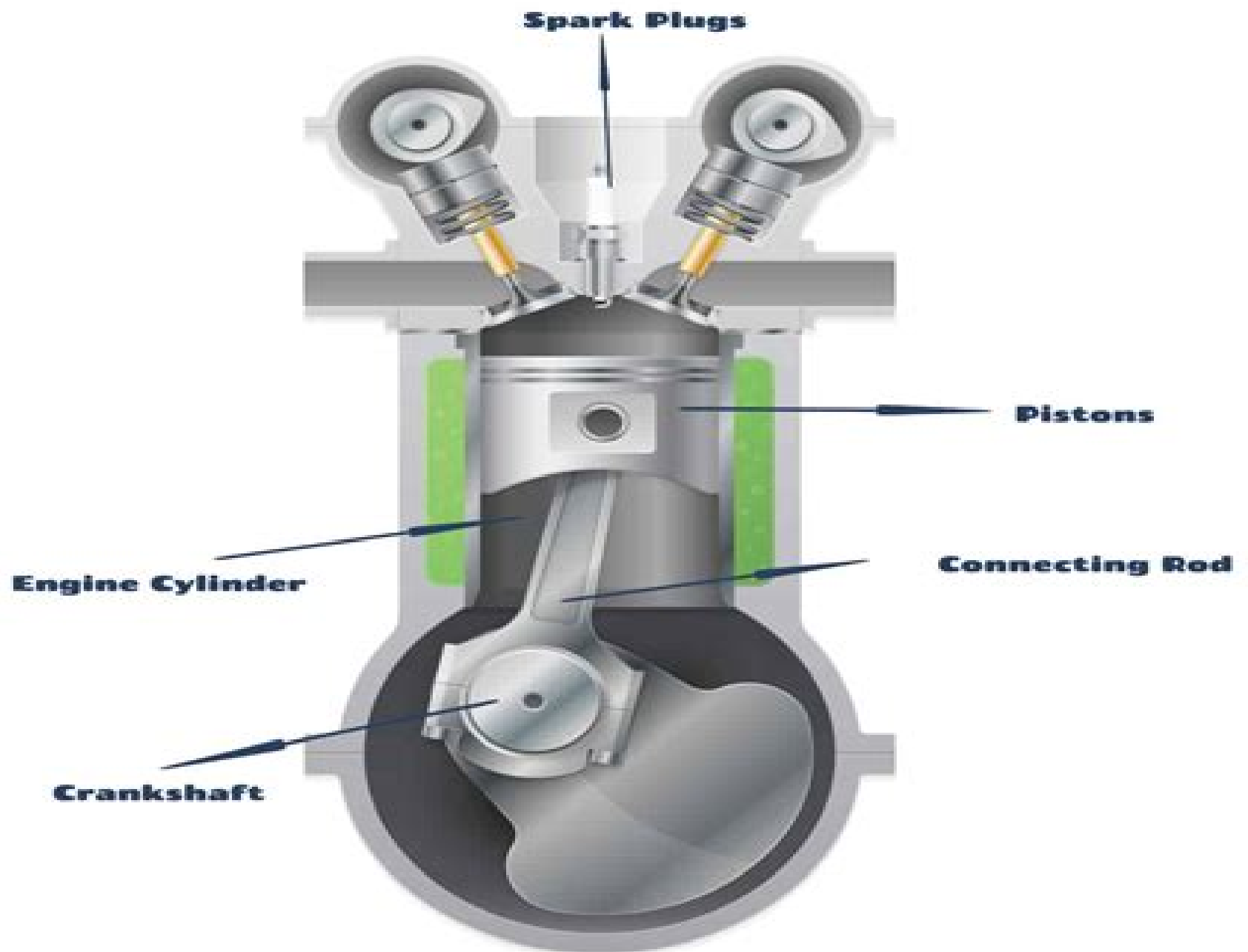
Core Components of Internal Combustion Engines
