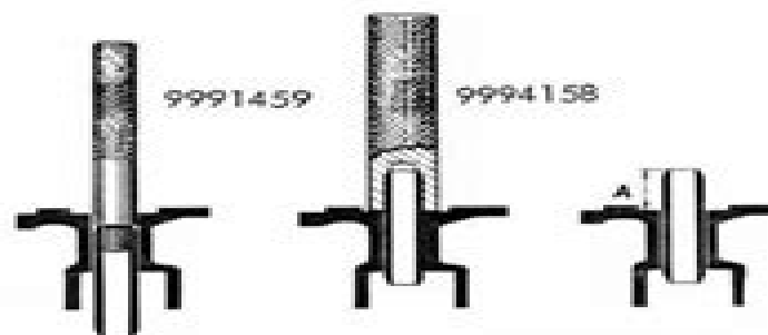
Fig. 12. Removing and fitting valve guides.
