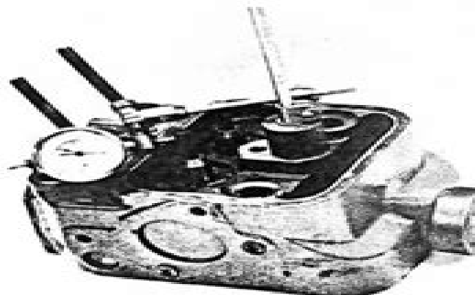
Fig. 11. Checking valve guide wear.
