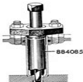
Fig. 9 Spreading the sleeve
