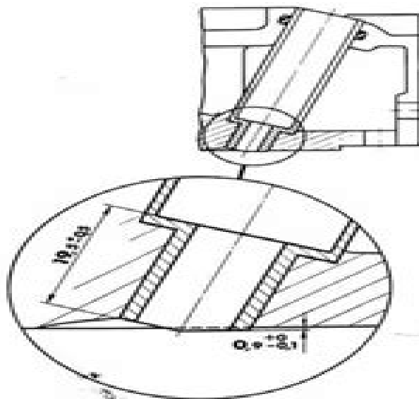
Fig. 10 Adjusting the sleeve
