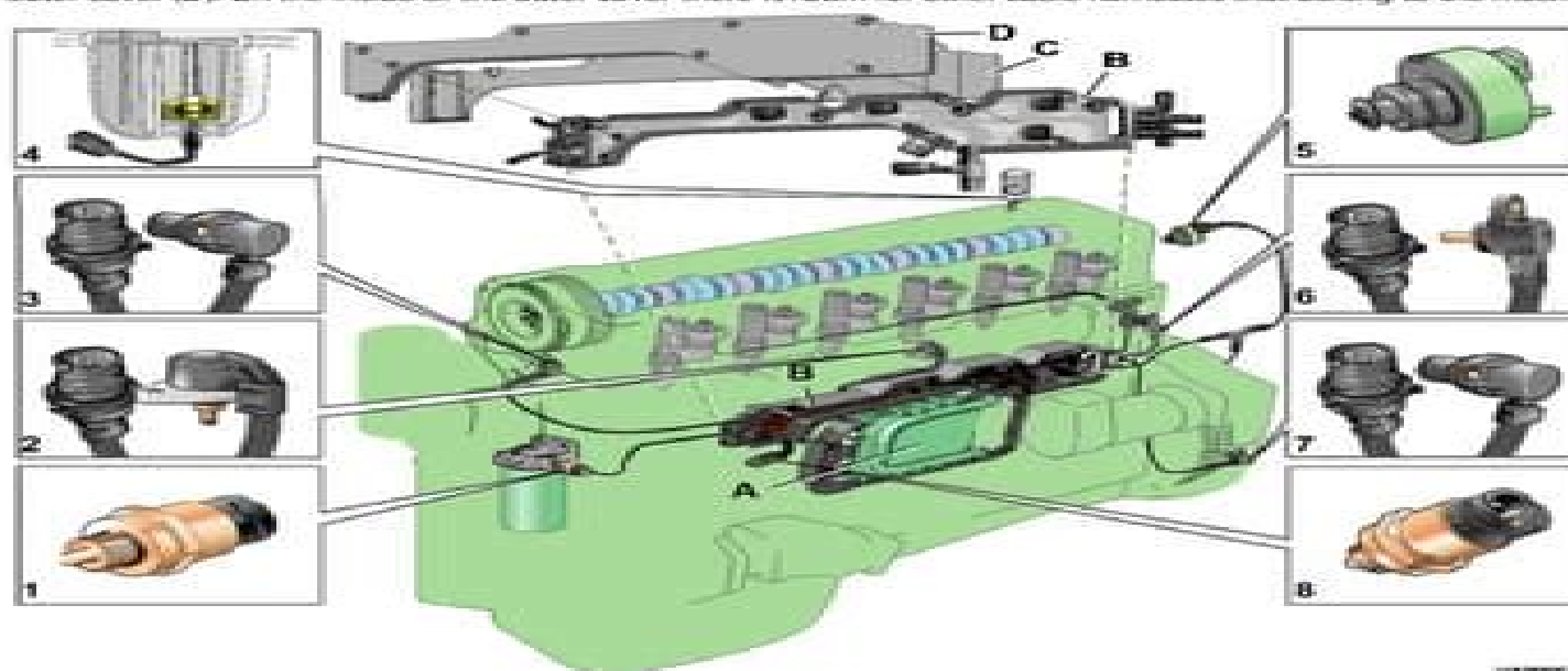
Figure 1 D12C, Engine sensors (some have dual functions)
