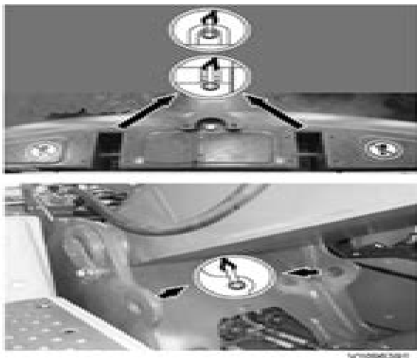
Figure 4 Lifting points NOTE!
