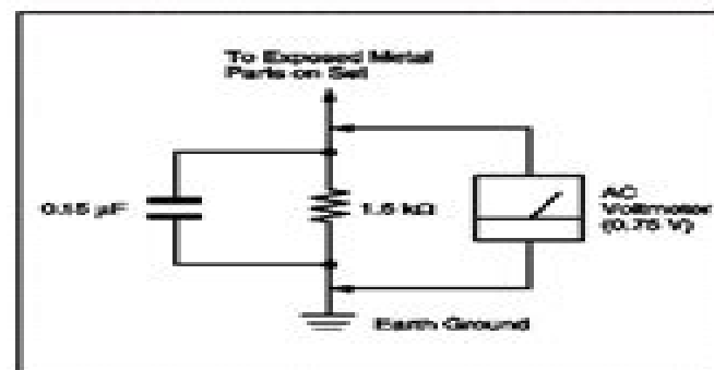
Fig. A: Use an AC voltmeter to check AC leakage
