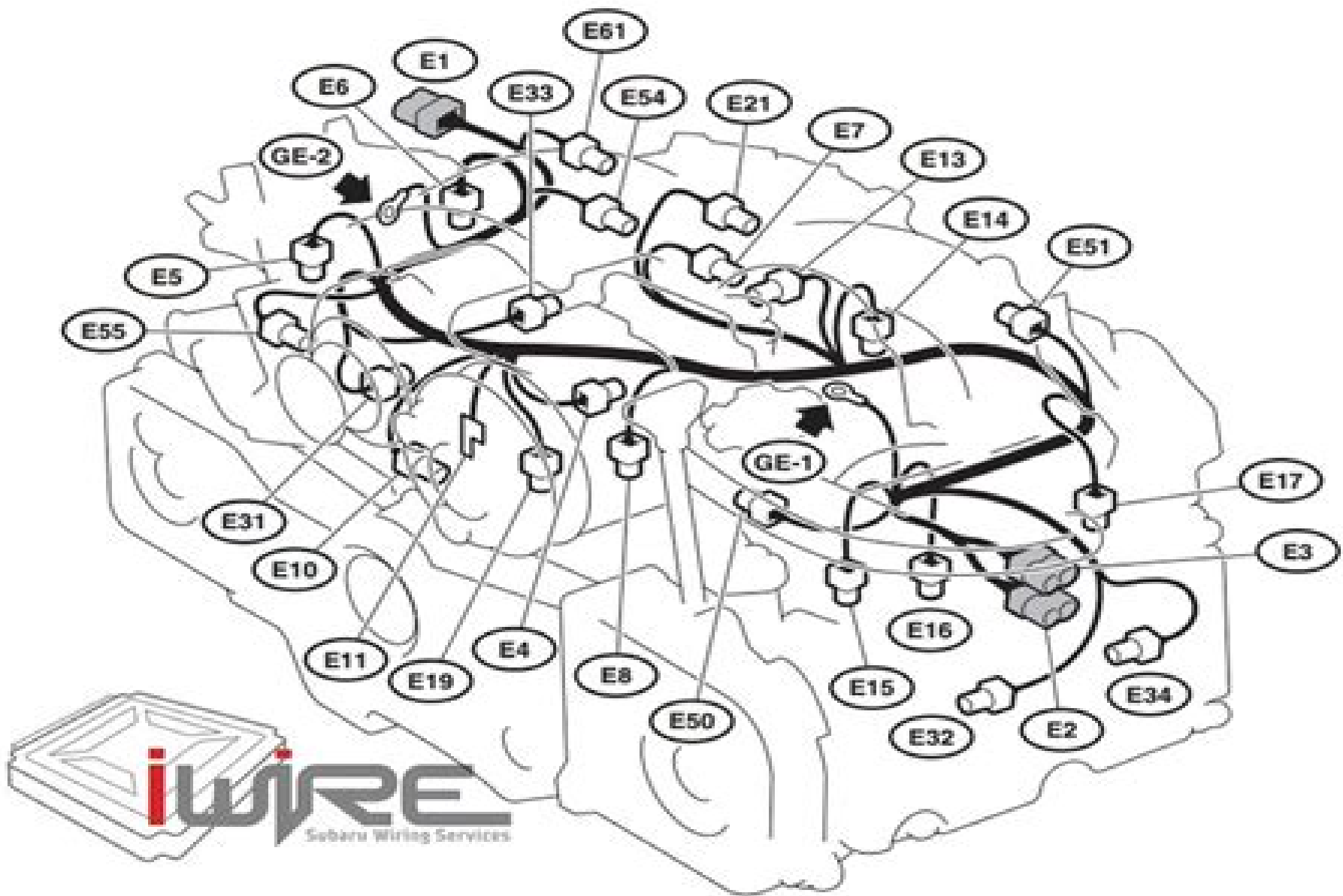
Engine Harness
