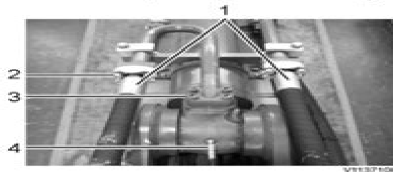
Figure 3752 Arm cylinder hydraulic hoses, removal
