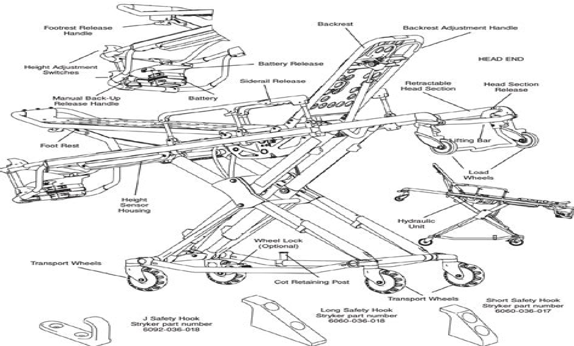
Figure 2: Cot Components
