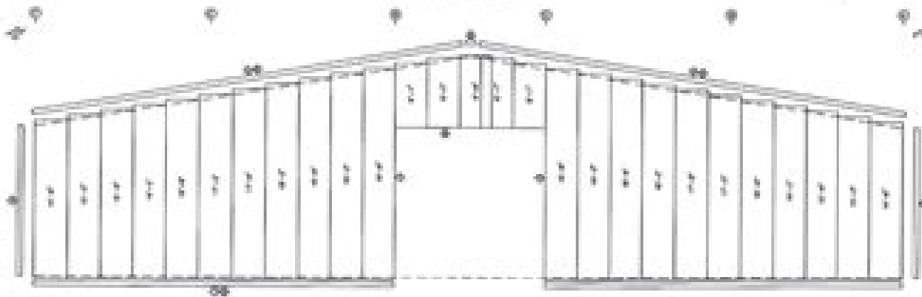
OVERALL SHEATHING & TRIM FRONT ELEVATION TRIM IS 1/2" X 4" X 8"
