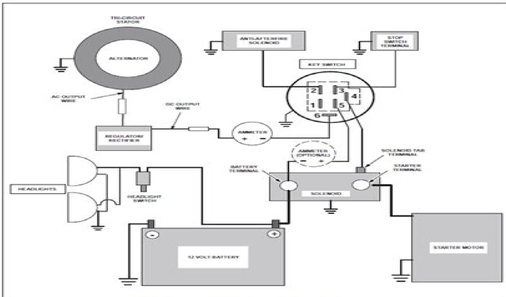
Typical 5/9 Amp Regulated Alternator Wiring Diagram With Charge Indicator Light 6 Pole Switch - Briggs & Stratton Part Number 6923-18
