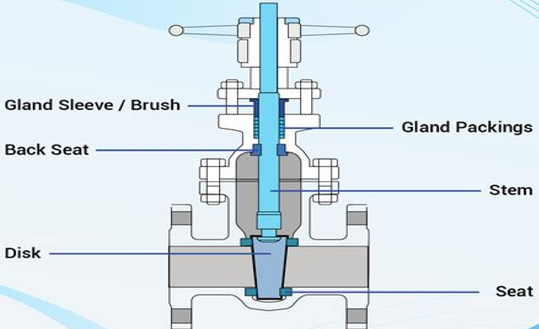
Valve Components
