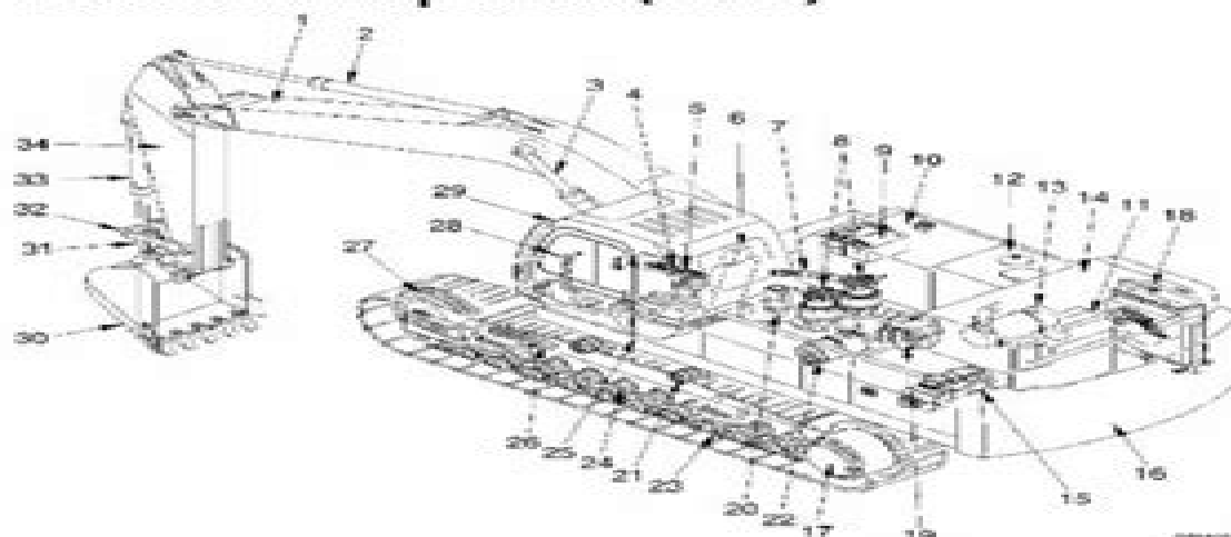
Figure 1 Location of components (EC460)
